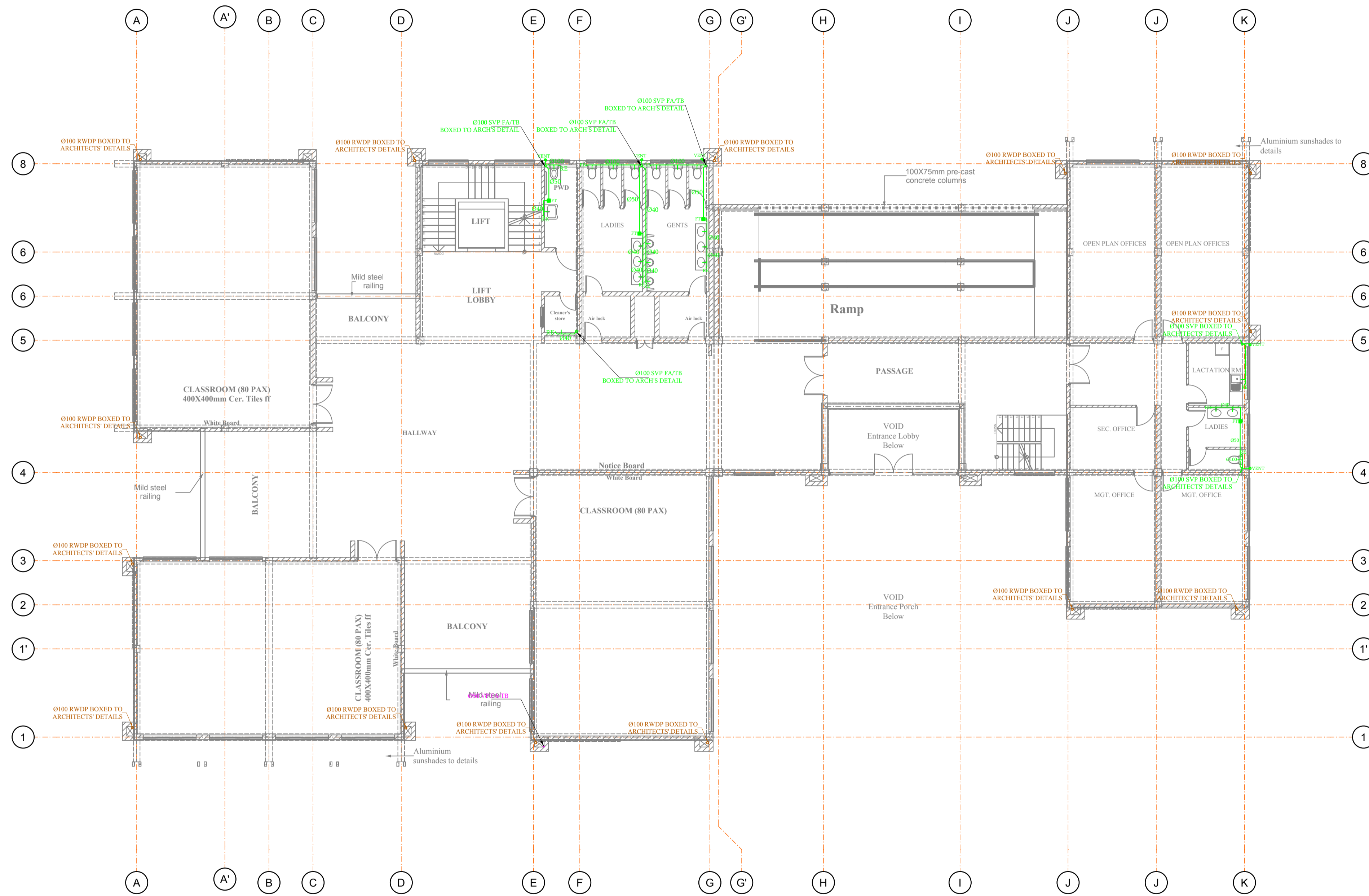
L[-]-J03 FIRST FLOOR PLAN SCALE 1:100
