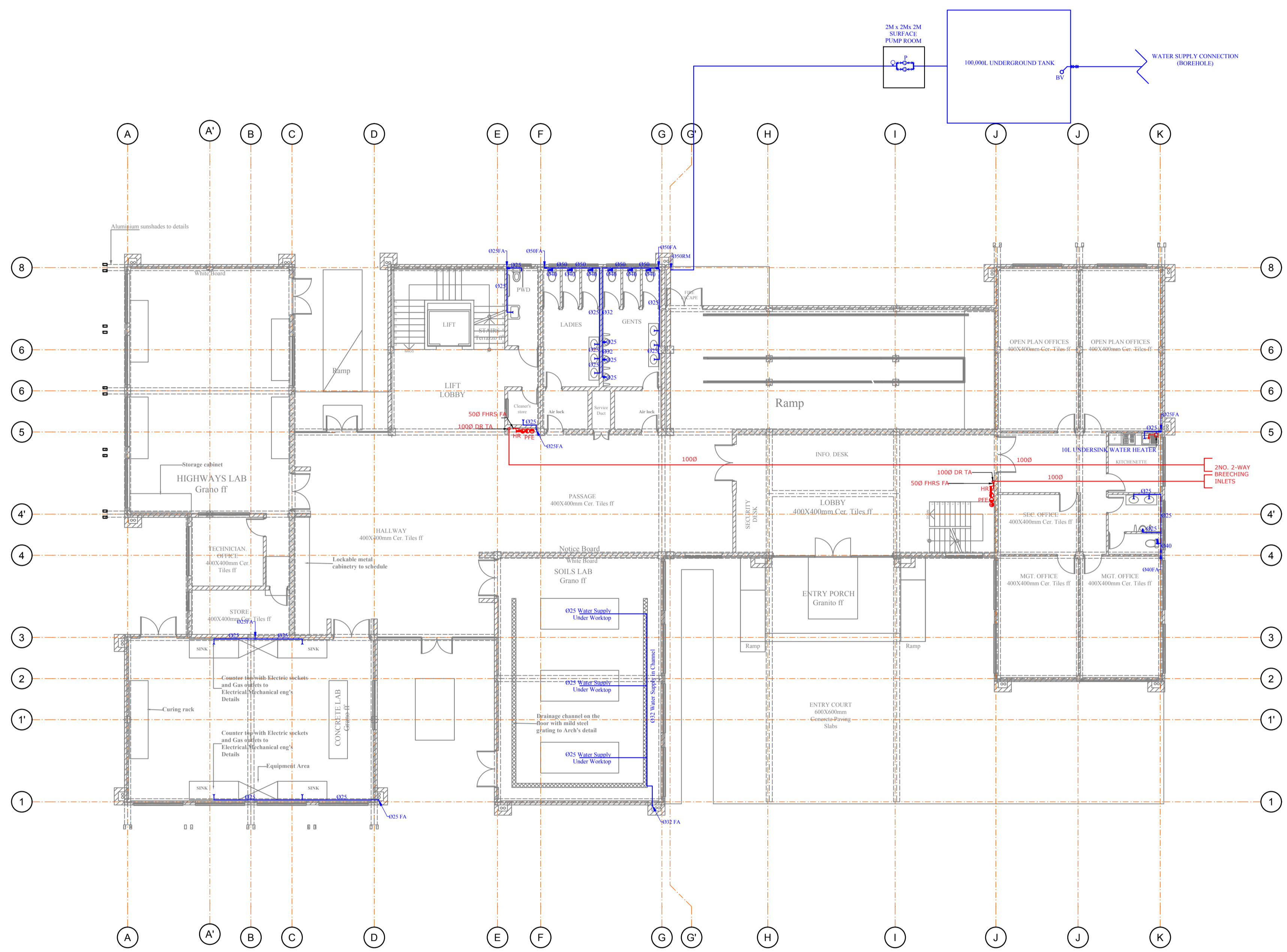
L1--02 GROUND FLOOR PLAN SCALE 1:100
