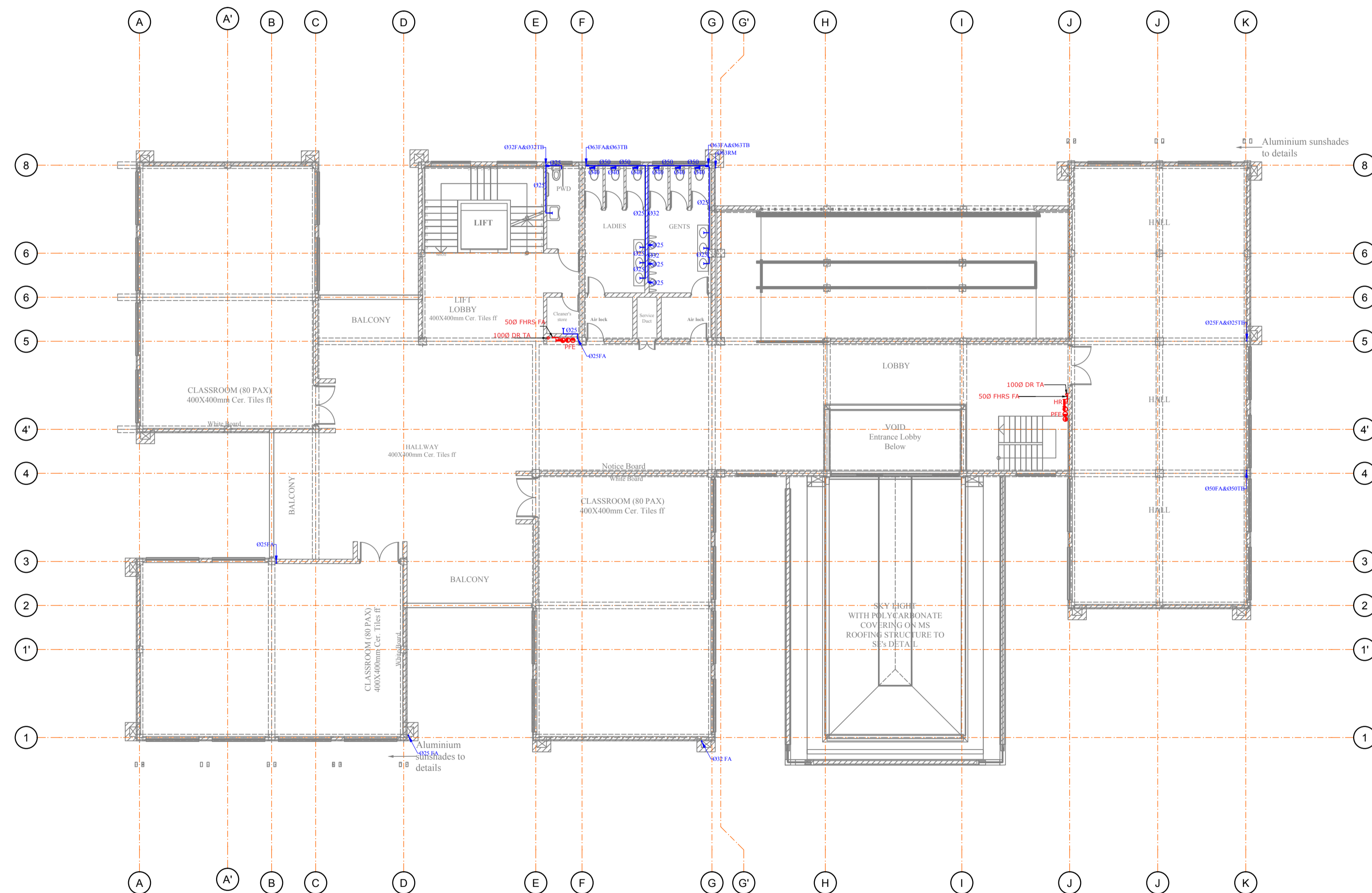
LJ-104 SECOND FLOOR PLAN SCALE 1:100
