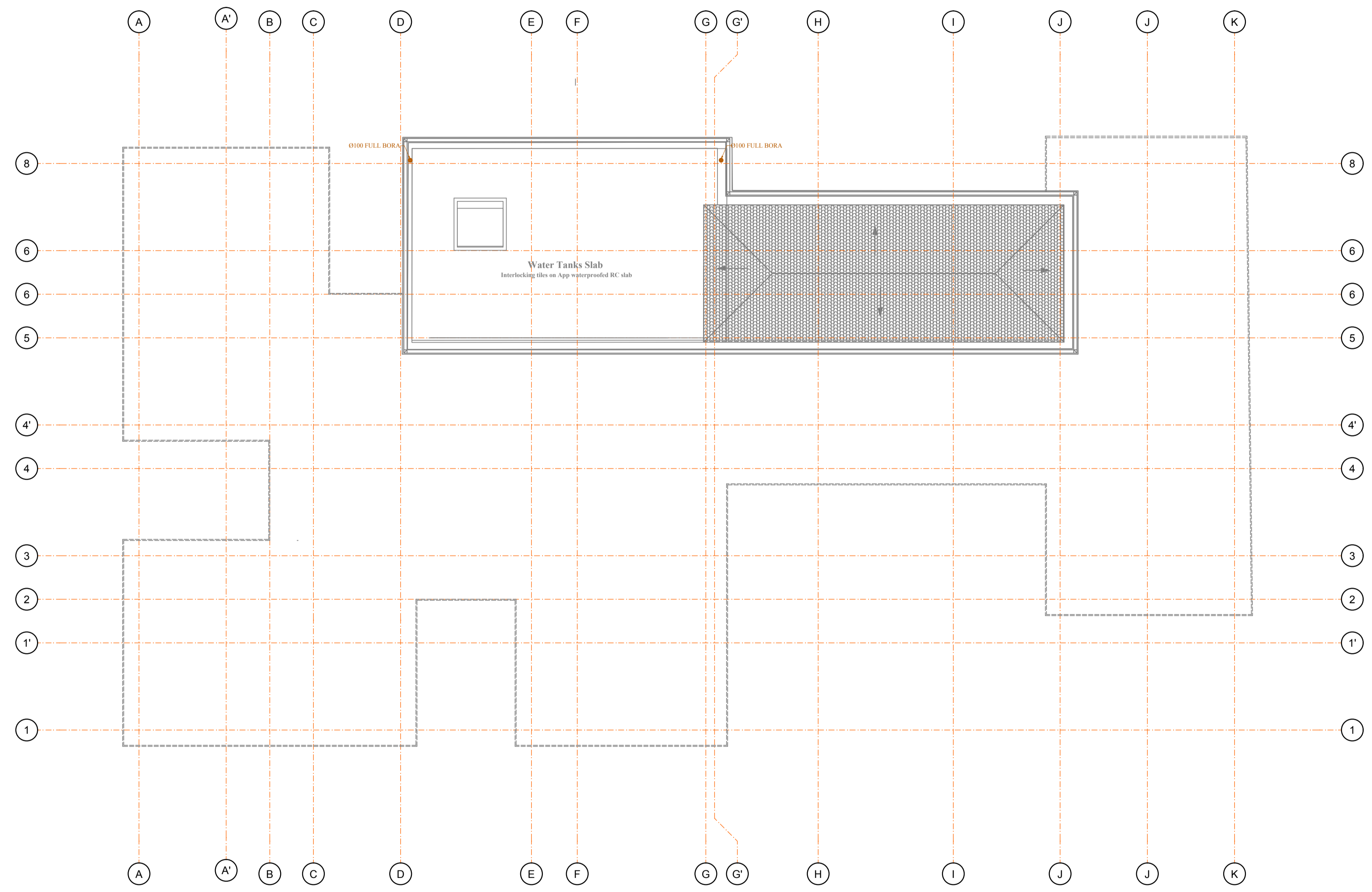
LJ-106 WATER TANK AREA & ROOF ABOVE RAMP SCALE 1:100
